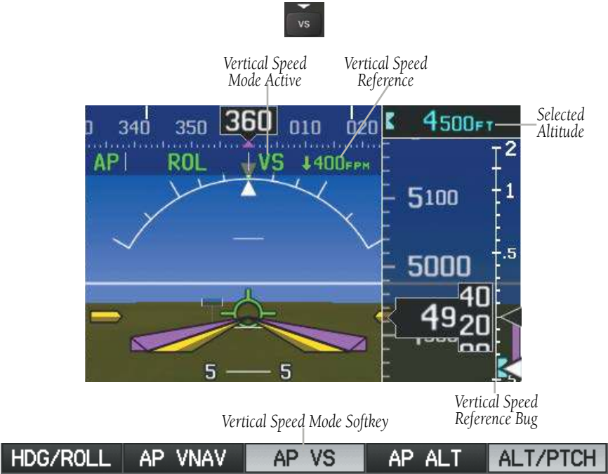
Vertical Speed Mode
