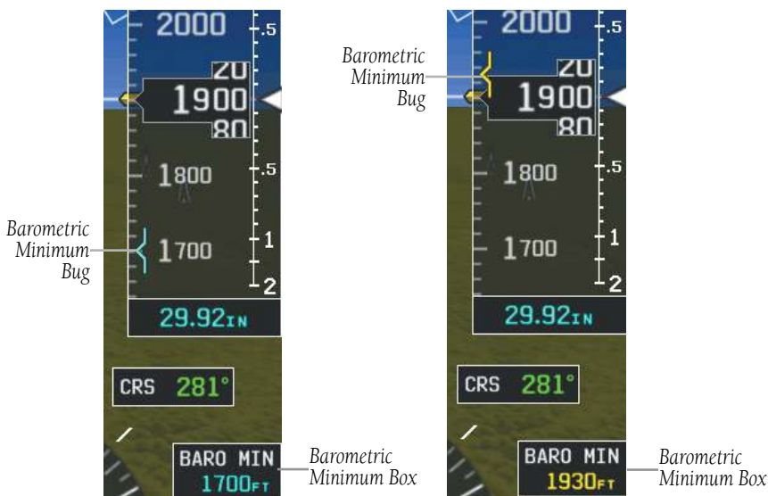
Barometric Minimum Visual Annunciations
