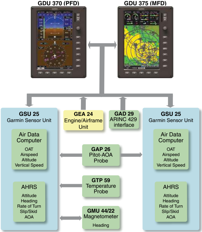
G3X Dual GSU 25 ADAHS
