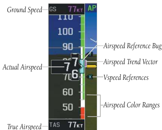
Airspeed Indicator
