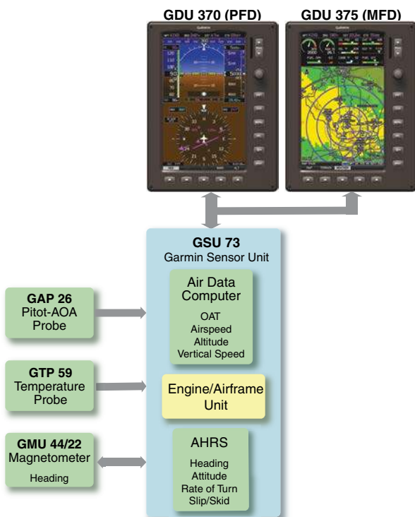
G3X Upgraded Panel (Full-Screen) (GSU 73)
