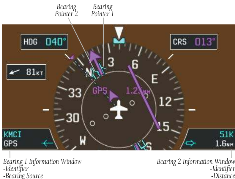
HSI with Bearing Pointers
