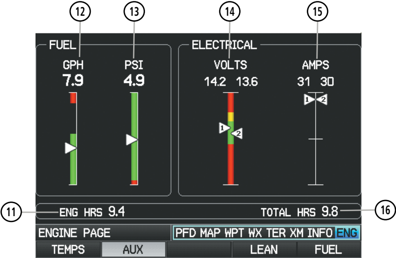
Example Engine (ENG) Page Configuration- AUX Softkey Selected (Split-Screen)
